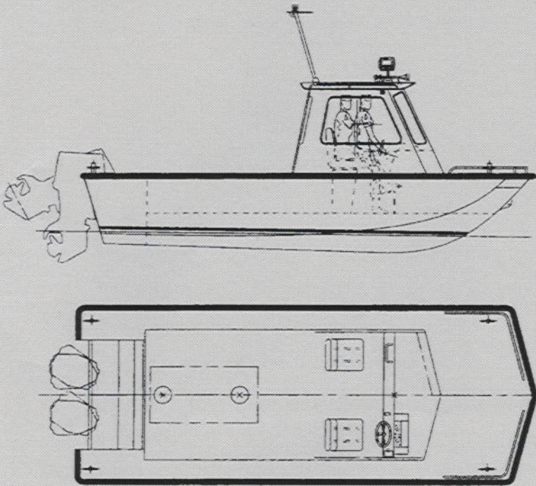
23' Little Giant with optional 10' survey cabin, air conditioner, emergency strobe light, aft wall with door, roof access ladder, flush aft deck, 3-tier safety railing and O/B platform with protection bar.
